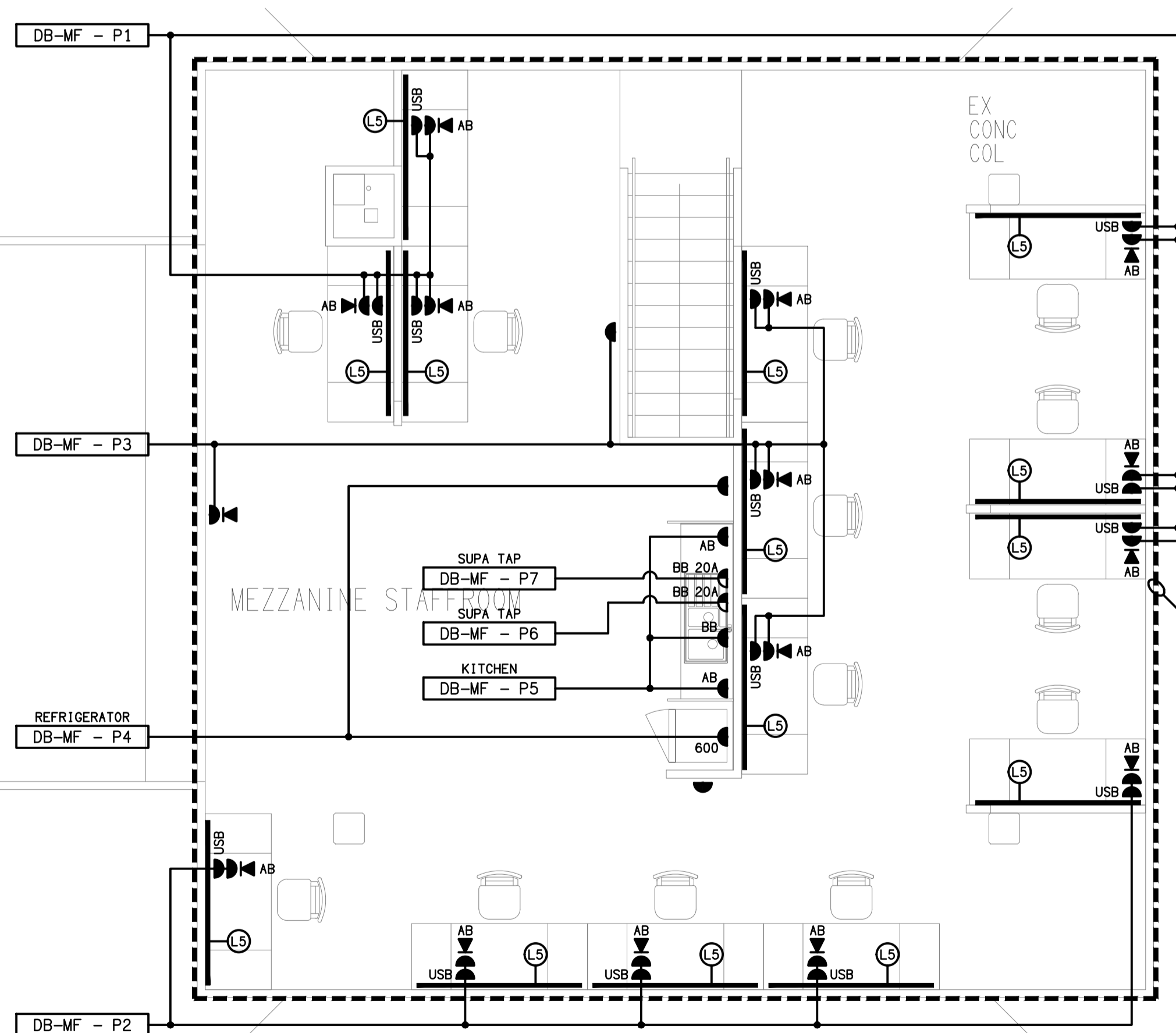
FLOOR PLAN PROPOSED MEZZANINE LEVEL SCALE 1:50
